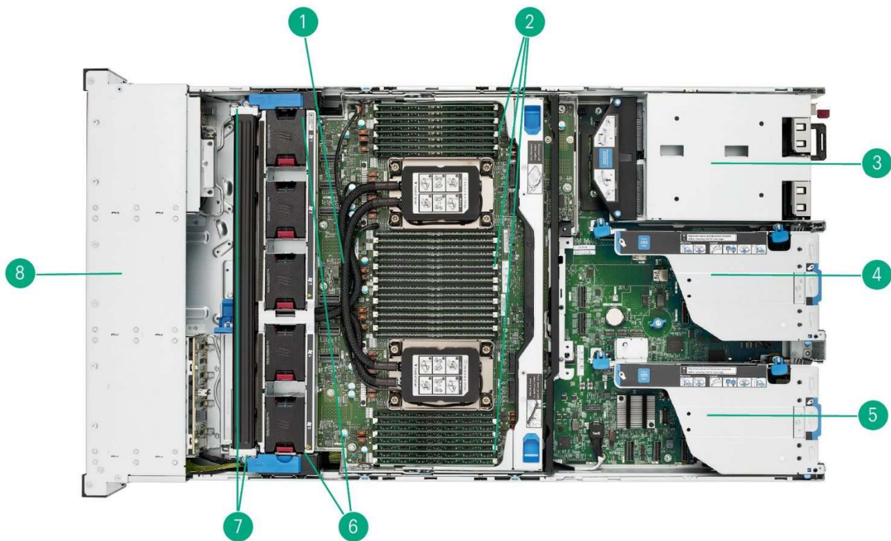
Internal View Liquid Cooling Chassis
