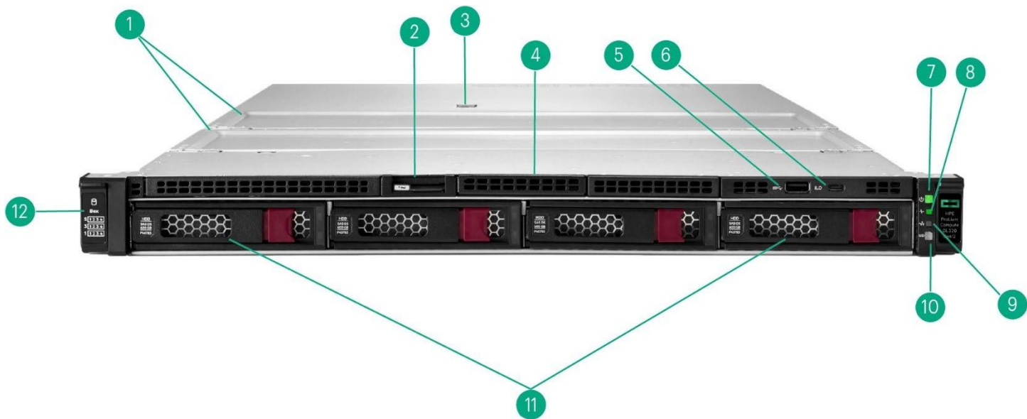
12 LFF Front View - 12 LFF + SAS drives shown
