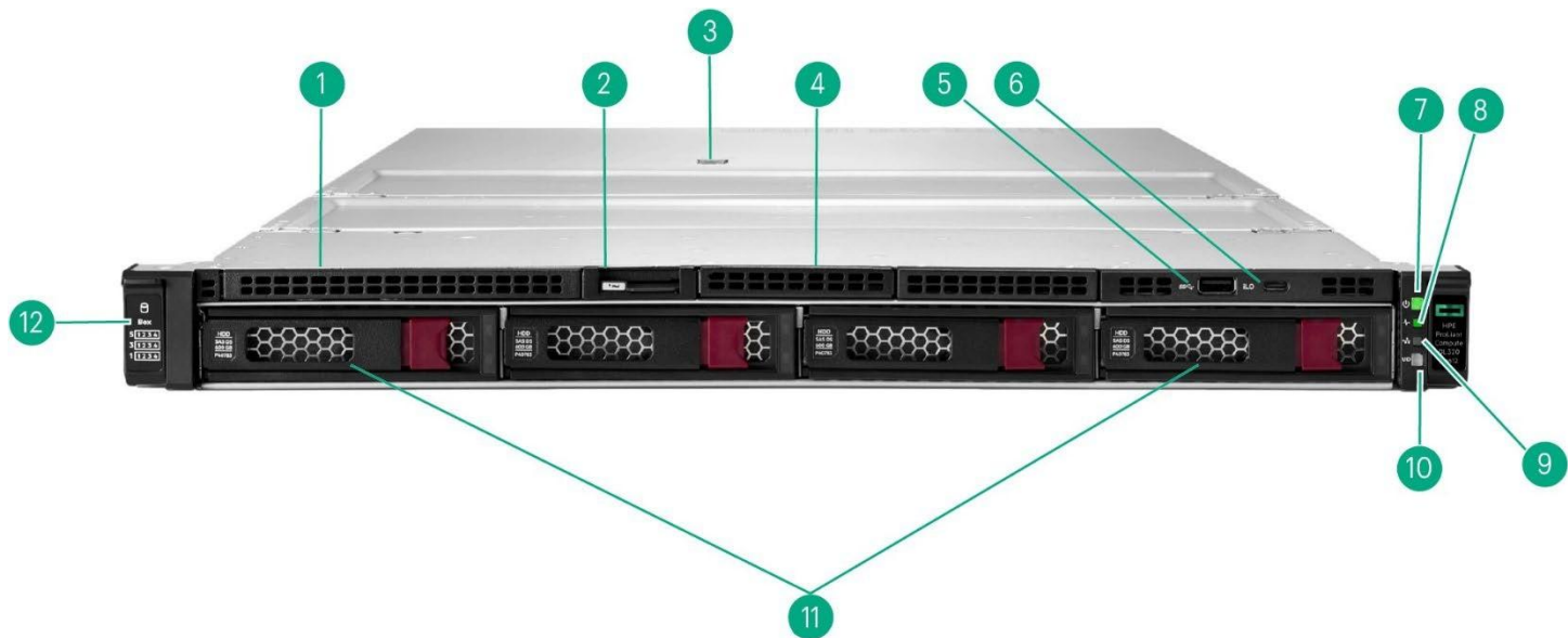
4 LFF Front View -- 4 LFF drives shown
