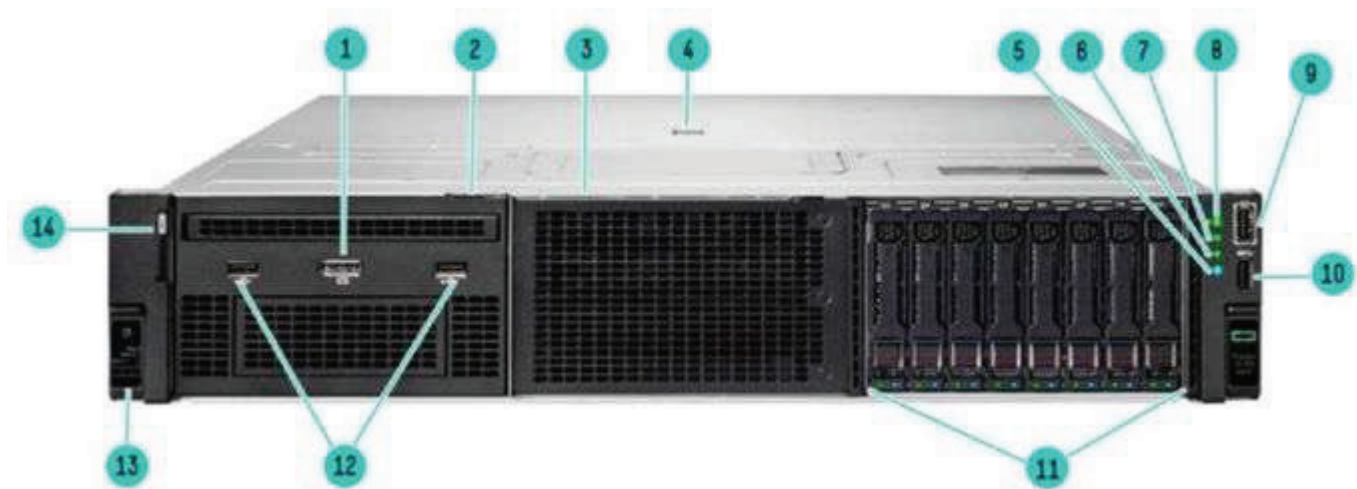
Front View - 8SFF chassis with optional Universal Media Bay shown
